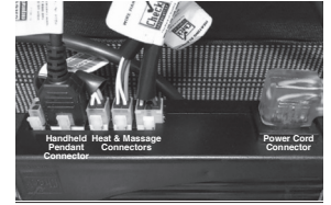
25 Heat and Massage Feature – Control Module and Transformer Unit Showing All Connections Correctly Made
